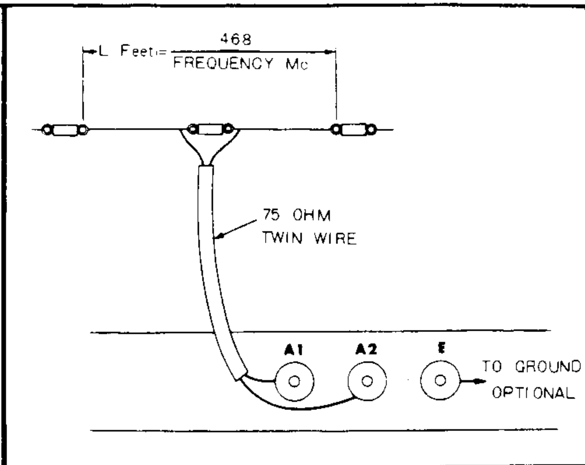
Figure 2. Doublet Antenna
